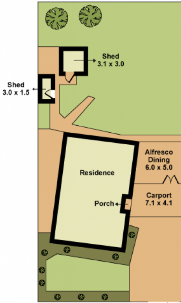
SITE PLAN
