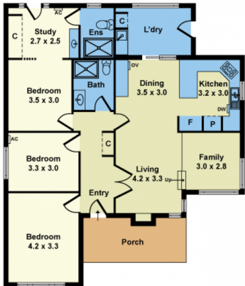
FLOOR PLAN
