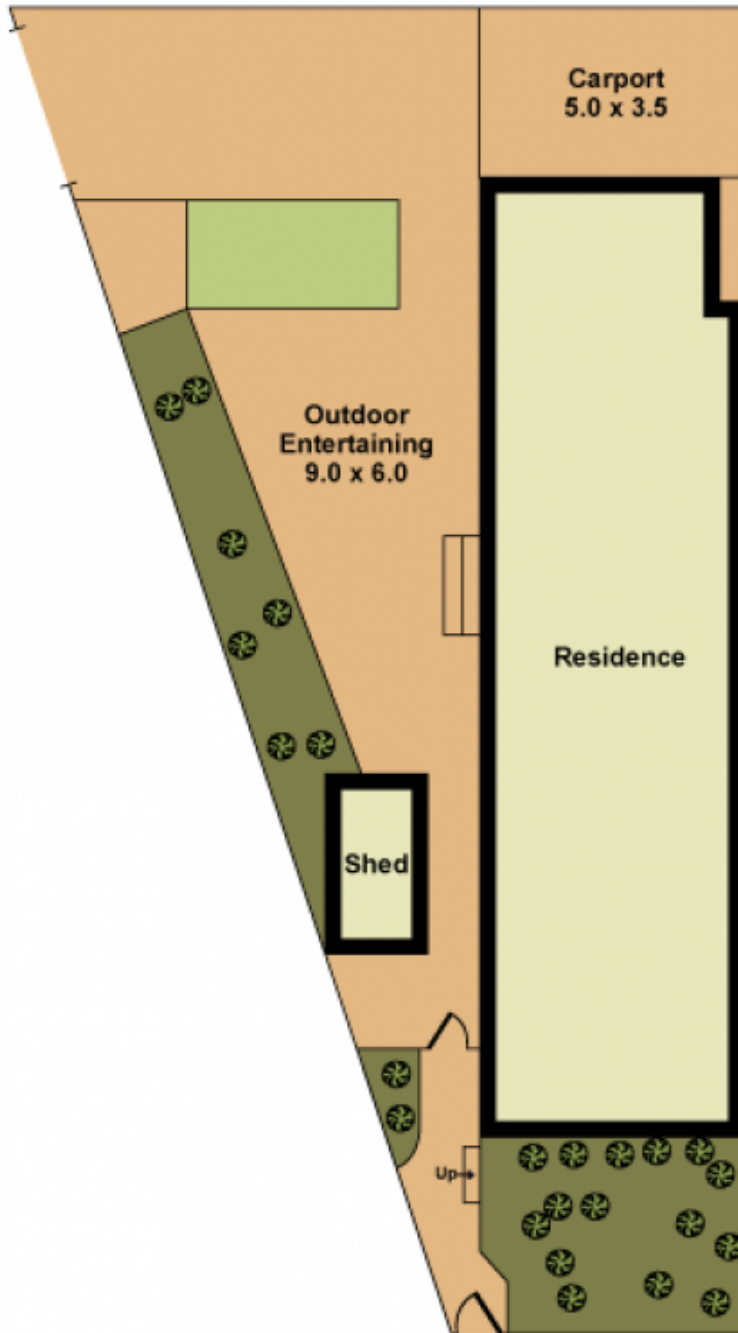
SITE PLAN
