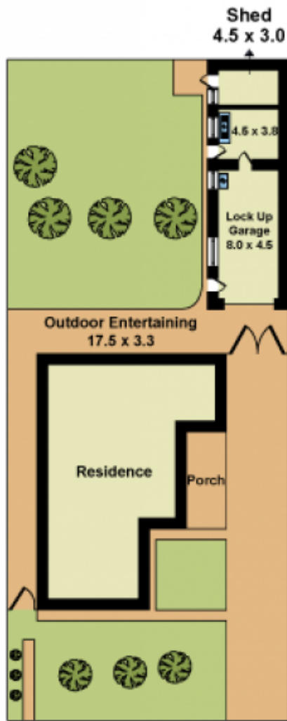
SITE PLAN
