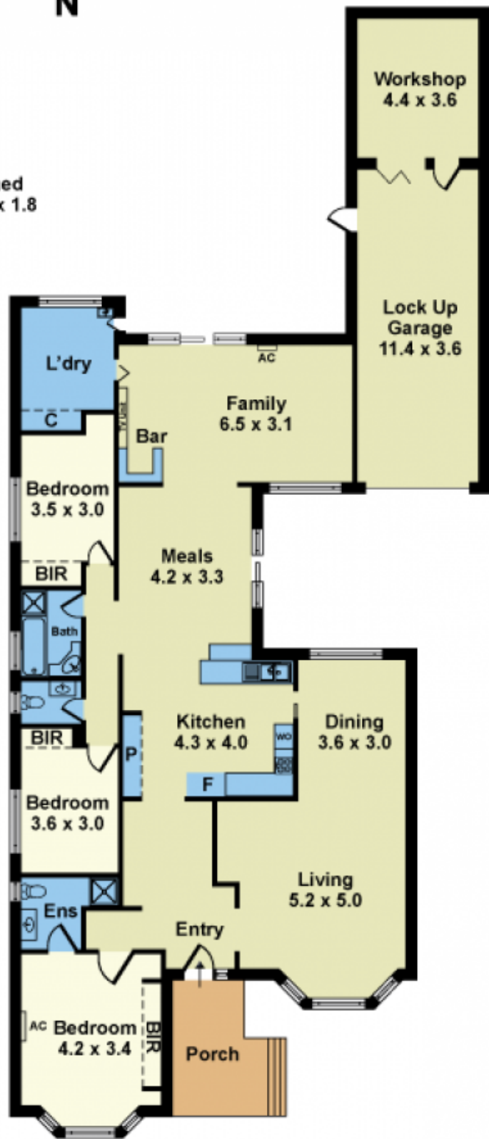
FLOOR PLAN
